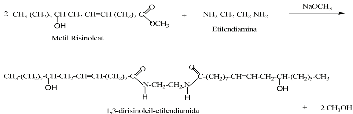
Gambar 1: Reaksi amidasi
